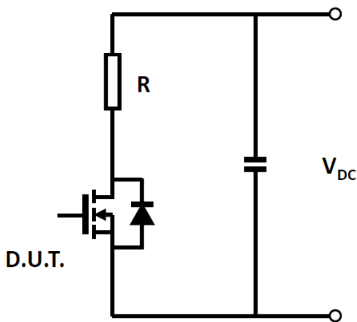
Figure 20. Schematic of Resistive Switching
