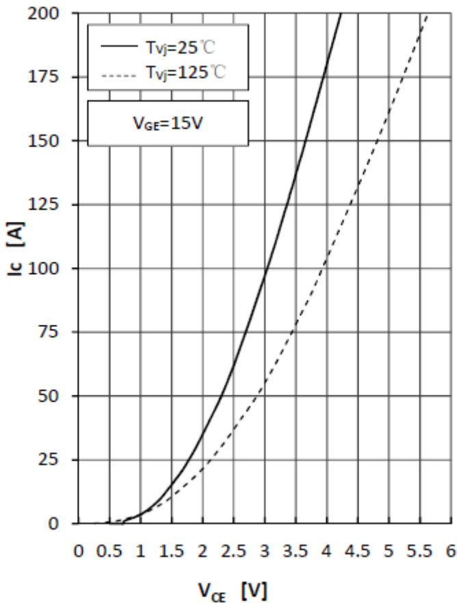
Fig1.IGBT Output Characteristics
