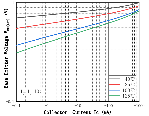
Fig.4 - Base-Emittor Voltage
